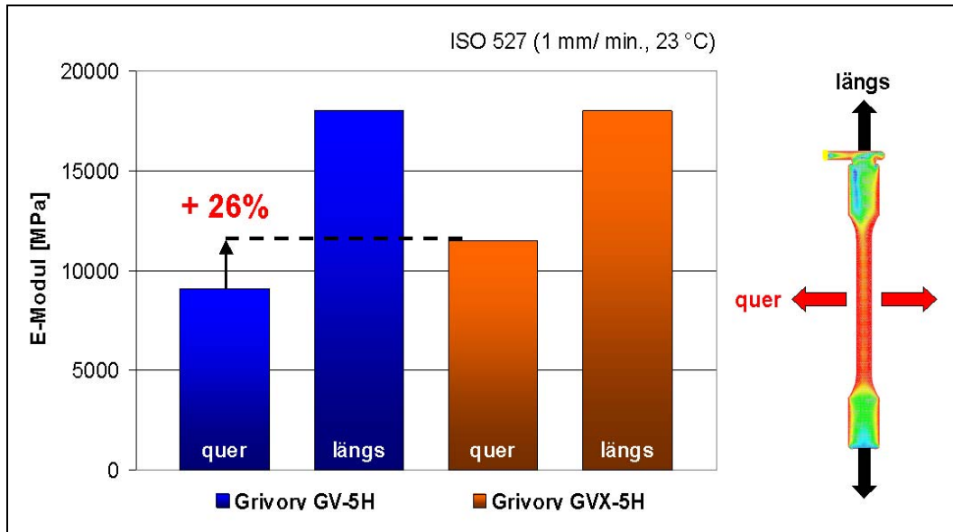
Fig. 1: Compared to standard products, Grivory GVX exhibits significantly higher transversal stiffness. (Picture: EMS-GRIVORY)
