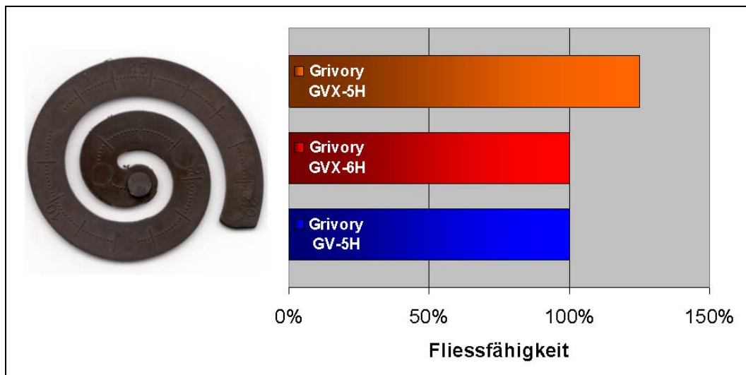
Fig. 2: Grivory GVX has improved flowability compared to standard products. (Picture: EMS-GRIVORY)
