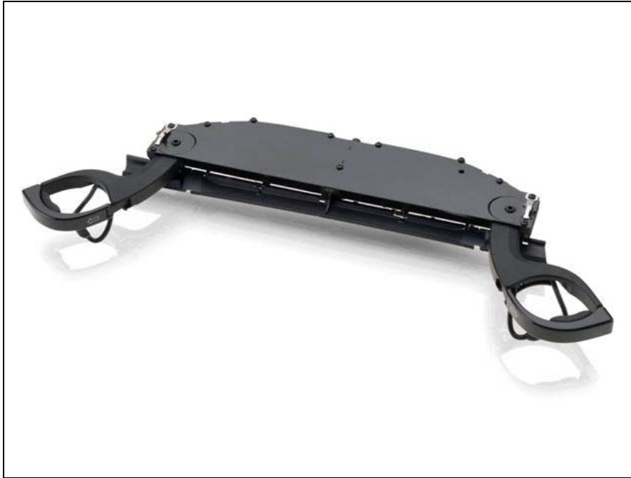
Fig. 3: Cup holder made by fischer automotive systems. Material: Grivory GVX-5H
